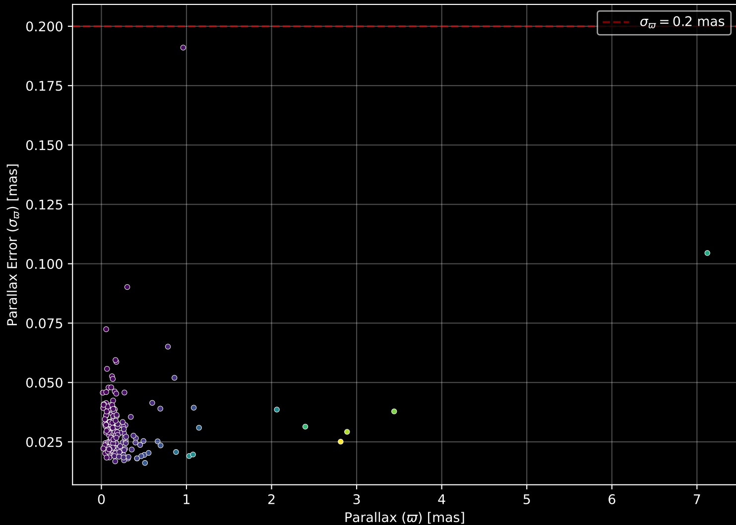
APOGEE DR17 Field: [000-08] Parallax Quality (n= 175)
