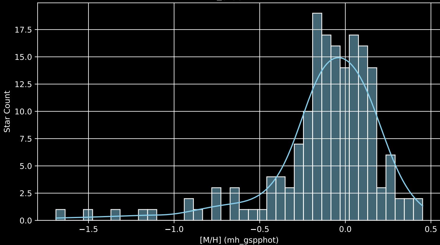
APOGEE DR17 Field: [000-08 [M/H] (mh_gspphot) (n= 173)
