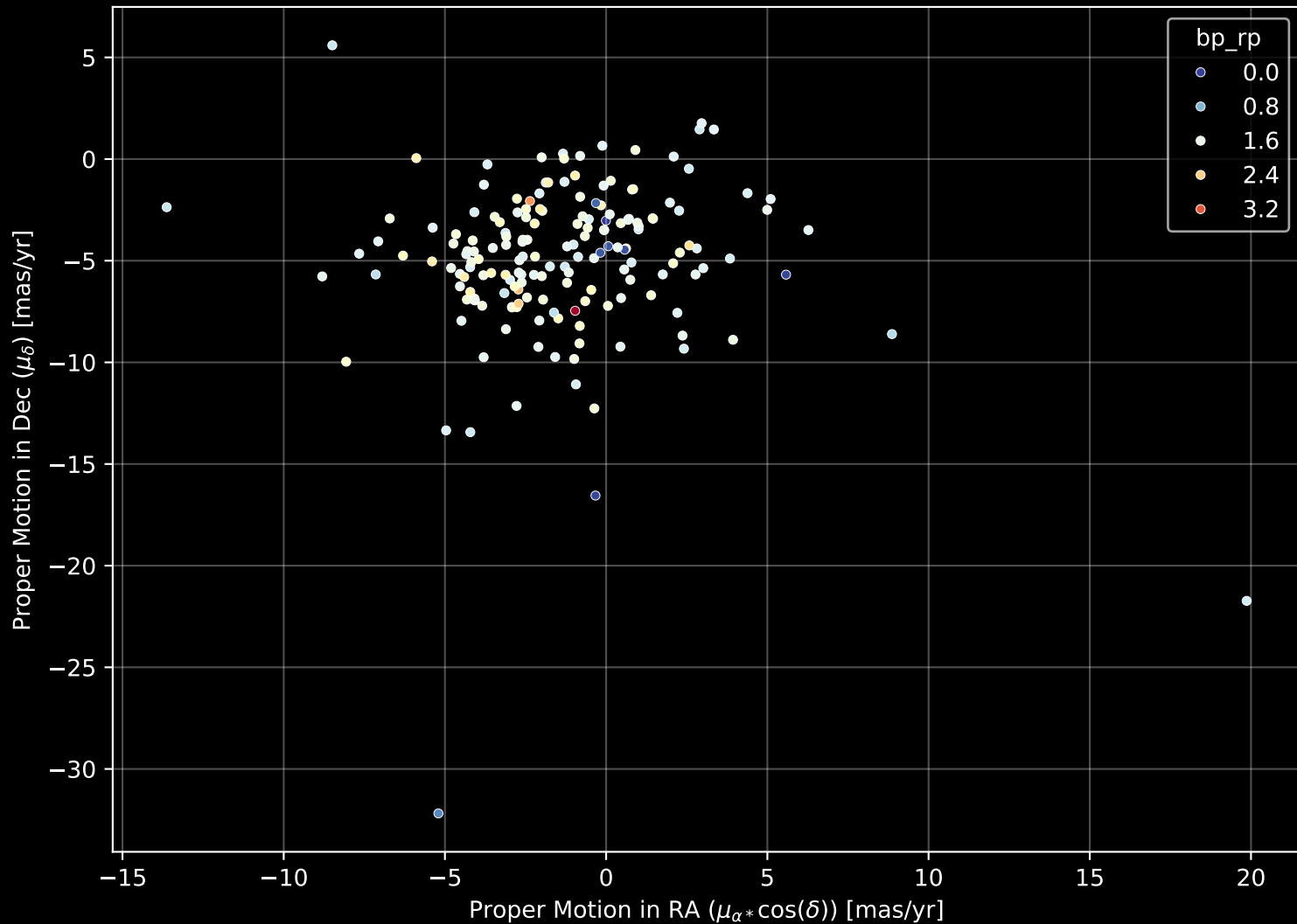
APOGEE DR17 Field: [000-08] Proper Motion Diagram (n= 175)
