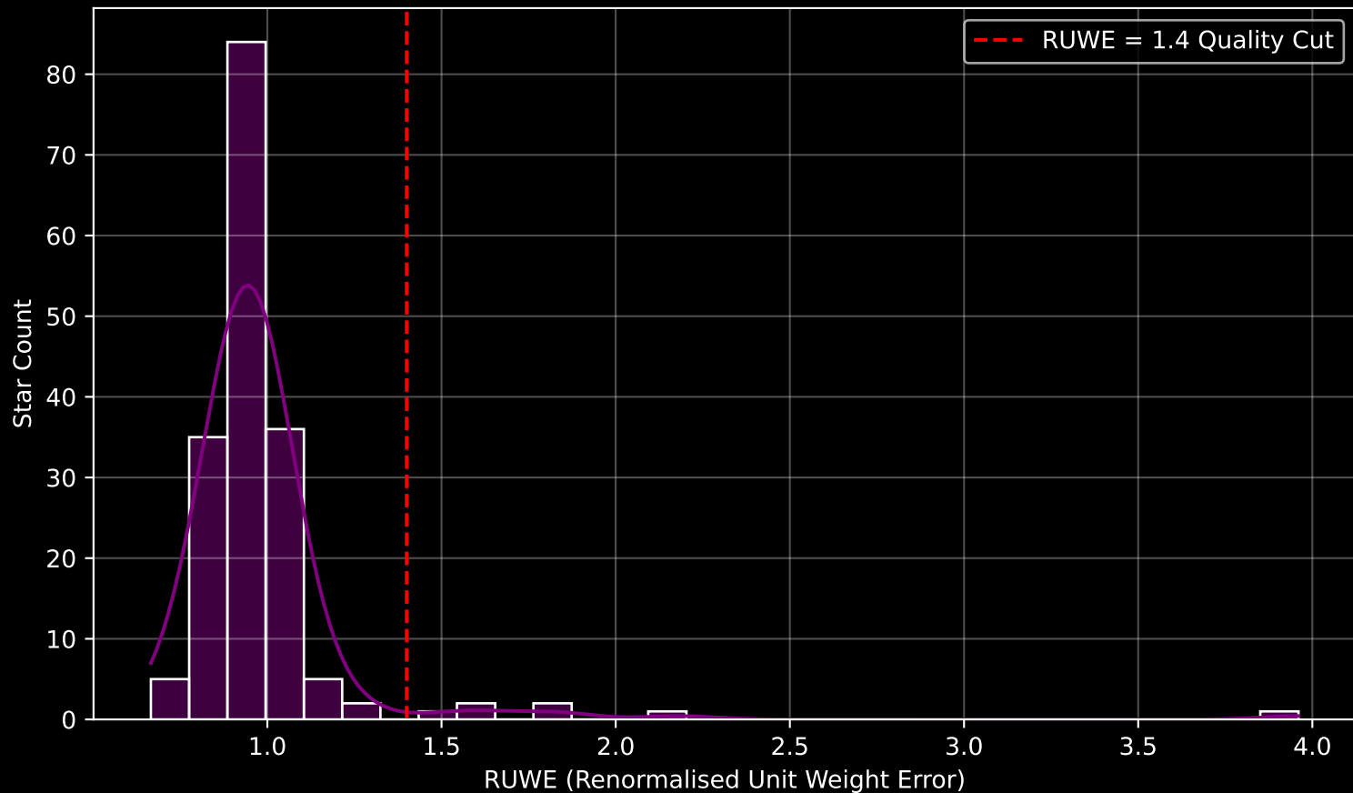
GAPOGEE DR17 Field [000-08] RUWE Distribution (n= 174)
